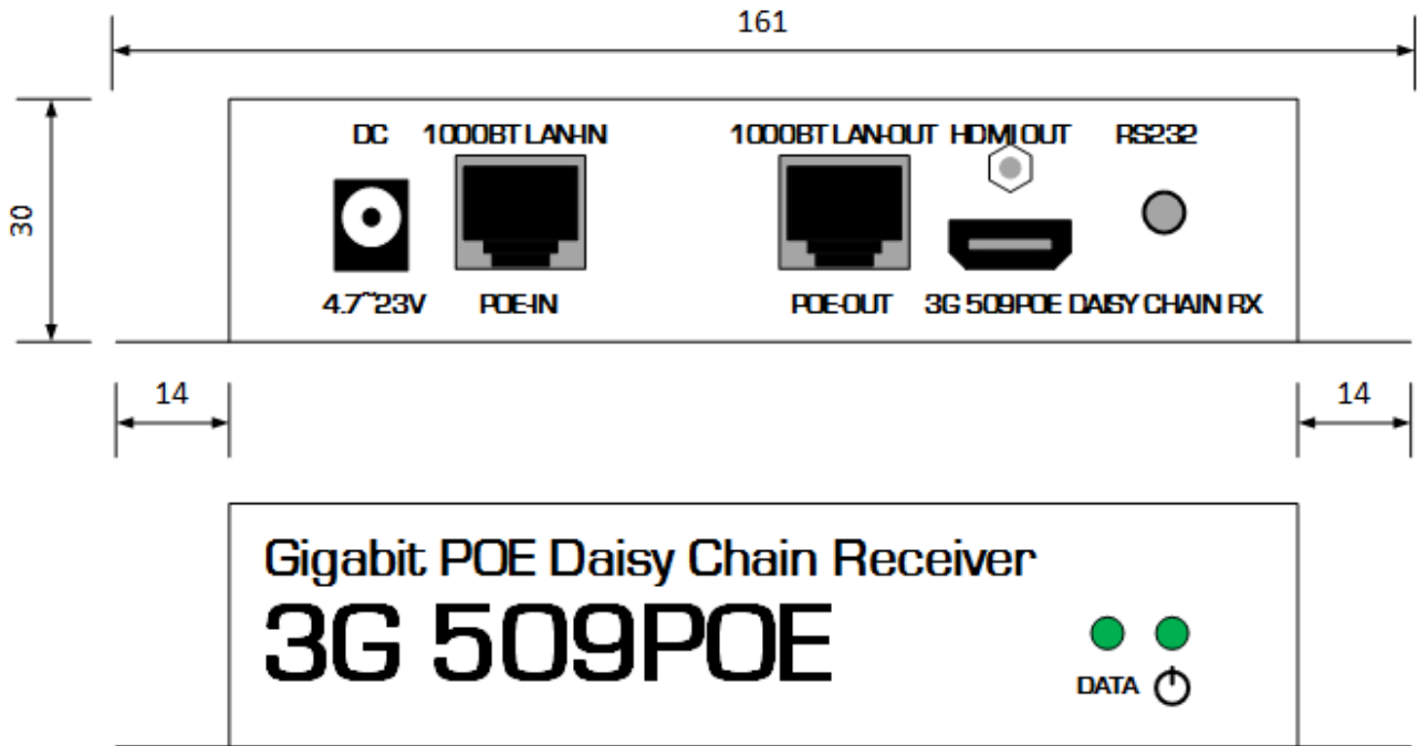
509POE Front/Back
